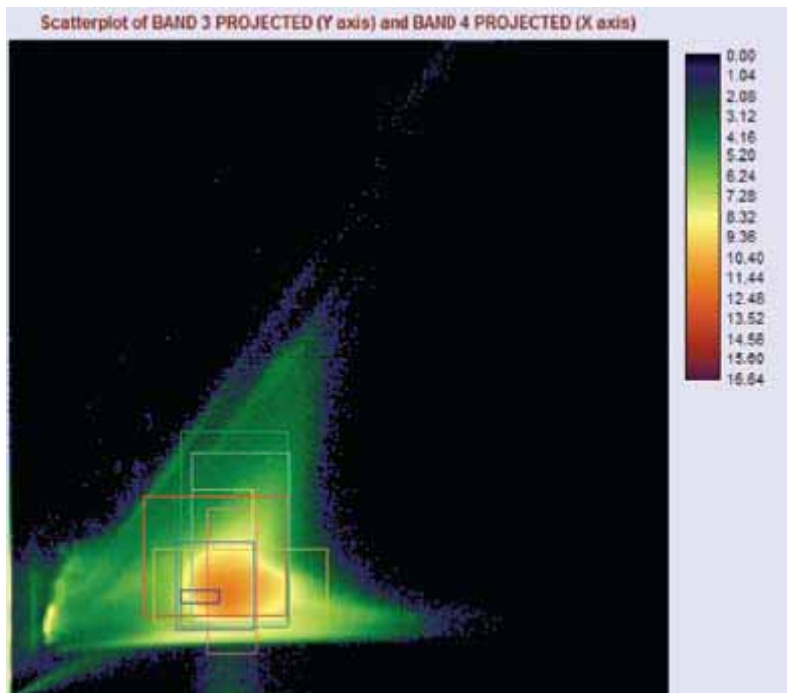
Fig 5: Scatterplot of Bands 3 and 4 with signature characteristic overlays.
