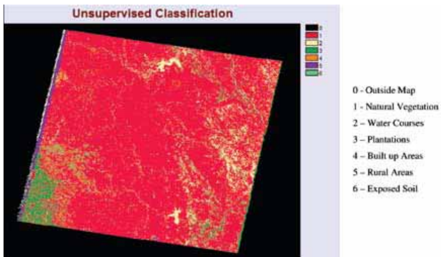
Fig 3: Land Cover Map using Cluster analyses in unsupervised classification.
