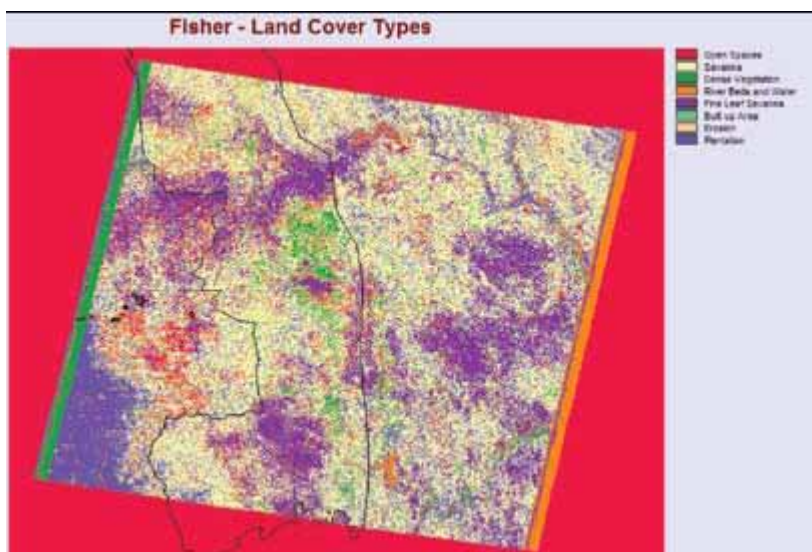
Fig 8: Final land cover map with outline of the Kruger National Park and training sites.
