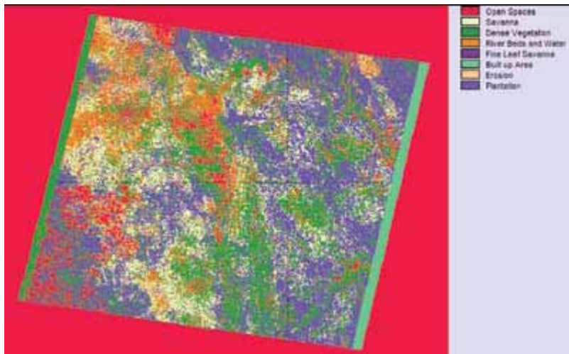
Fig 6: Image classification using Mindist classification.
