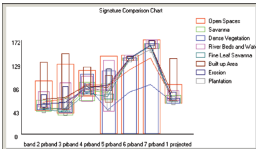
Fig 4: Graph displaying the land cover types and their relative reflectance values across each Landsat TM band.
