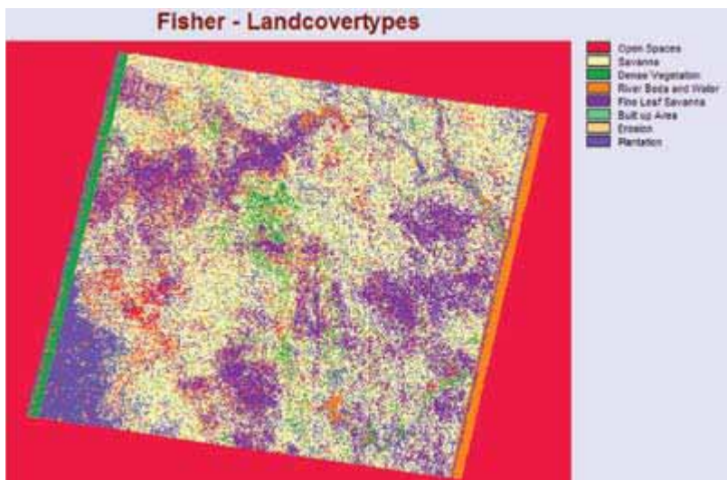
Fig 7: Image classification using Fisher module.
