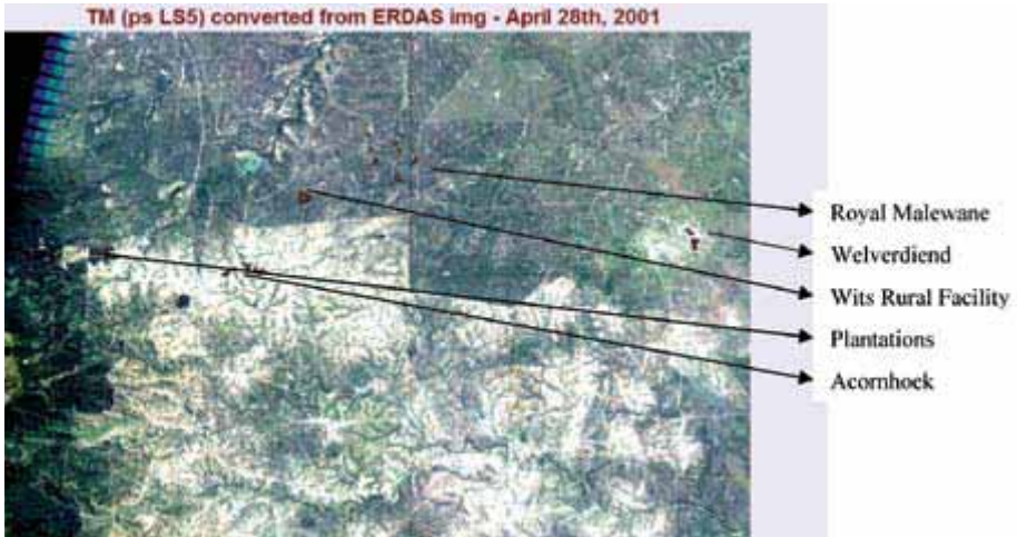
Fig 2: The full cover image of the research area showing the 58 training sites from the five different research areas.
