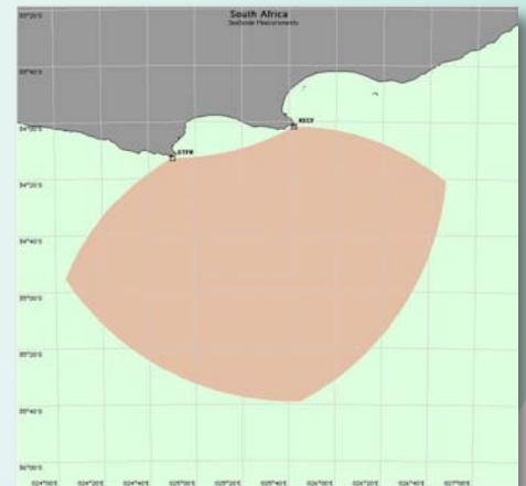
A map showing the radial range of measurement (180 km) of the SeaSonde HR radar. Image credit: Andrés Alonso-Martirena (CODAR Europe)
