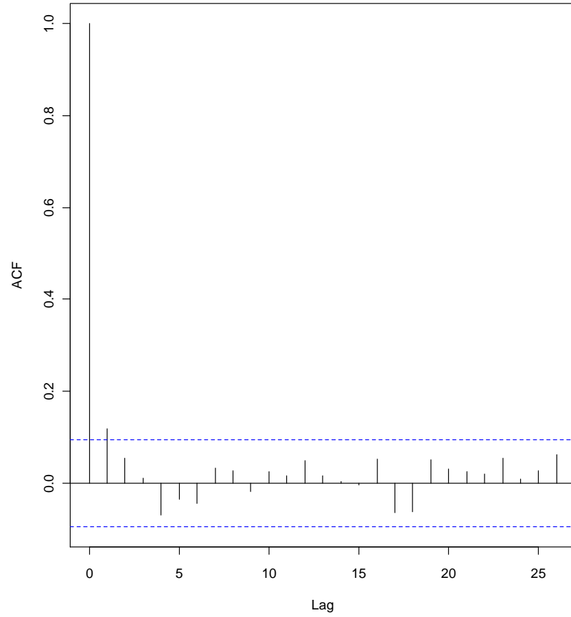
Bassonskloof Farm 1976 - 2011 Autocorrelation Function
