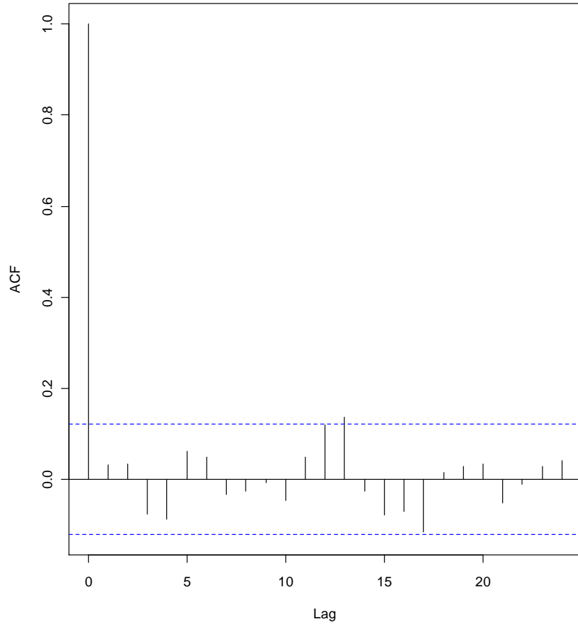
Figure 3 - Rainfall autocorrelation
